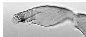
Two-segmented tarsus
