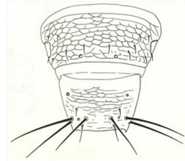
Tergites VIII-IX
