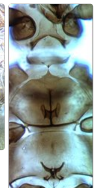
Thoracic sternites
