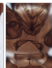
Prosternum
